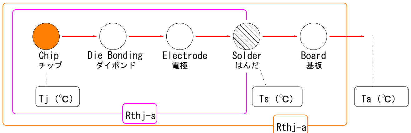
Figure 2 Flow chart of the heat from the chip
