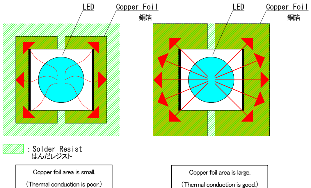
Figure 8 Copper foil pattern shape of the printed circuit board
