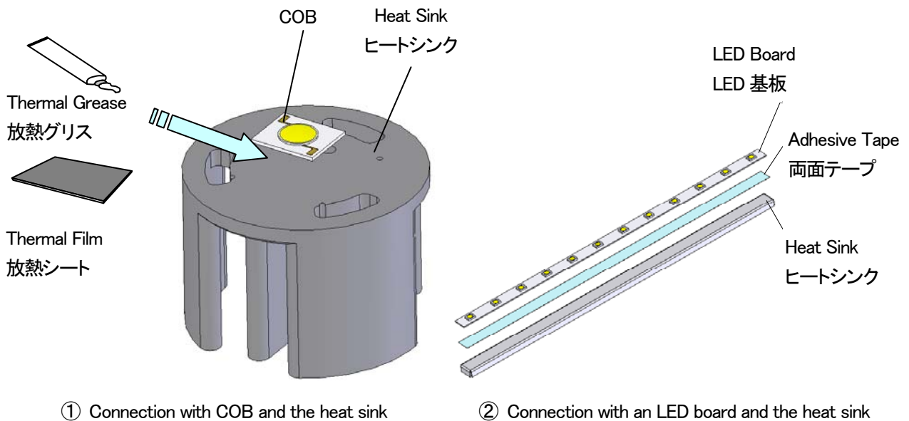
Figure 11 Connection with the board and the heat sink
