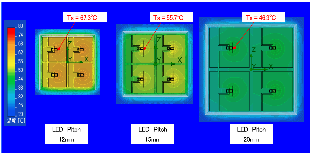
Figure 10 Thermal distribution simulation results (Example: NSSW157)
