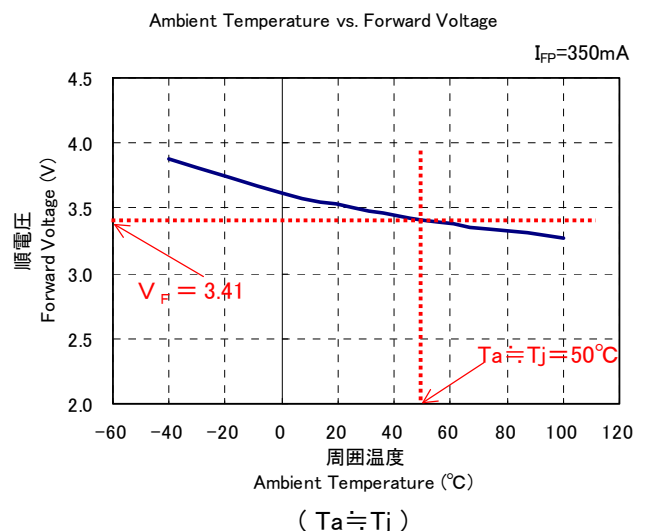
Figure 5 Calculation of T_j (NS3W183)
