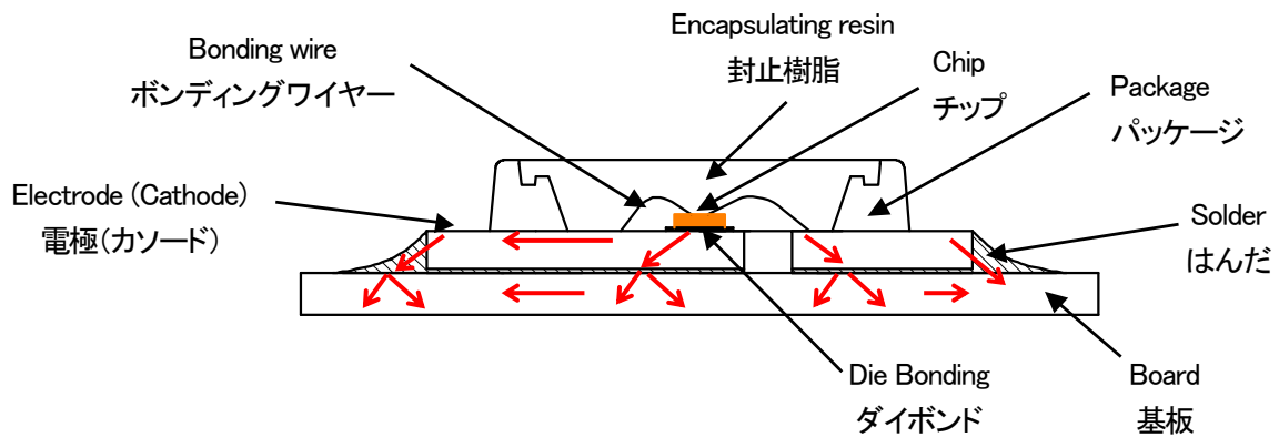
Figure 1 LED's structure and an example of the heat path (Example LED Model: NS3W183)
