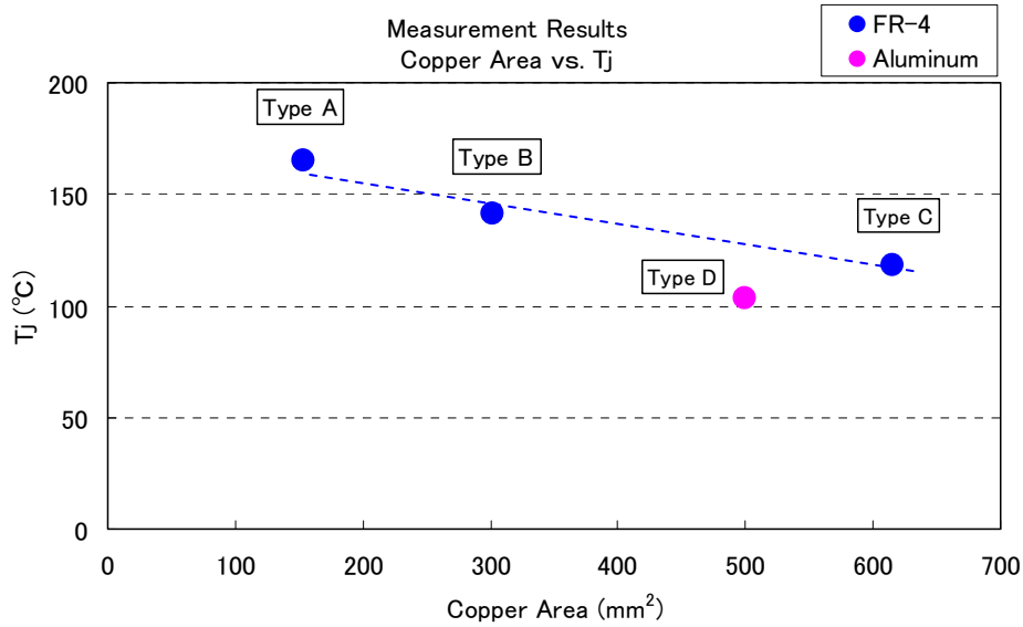
Figure 7 Thermal Measurement Results for NS6W183 (Copper area vs Tj)
