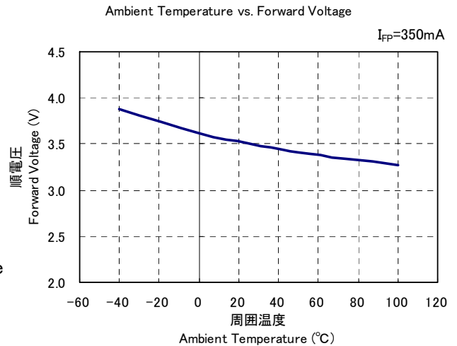
Figure 4 Ambient Temperature vs. Forward Voltage (NS3W183)
