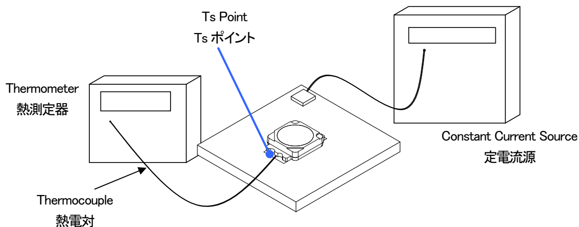
Figure 3 Thermal Measuring Set Up
